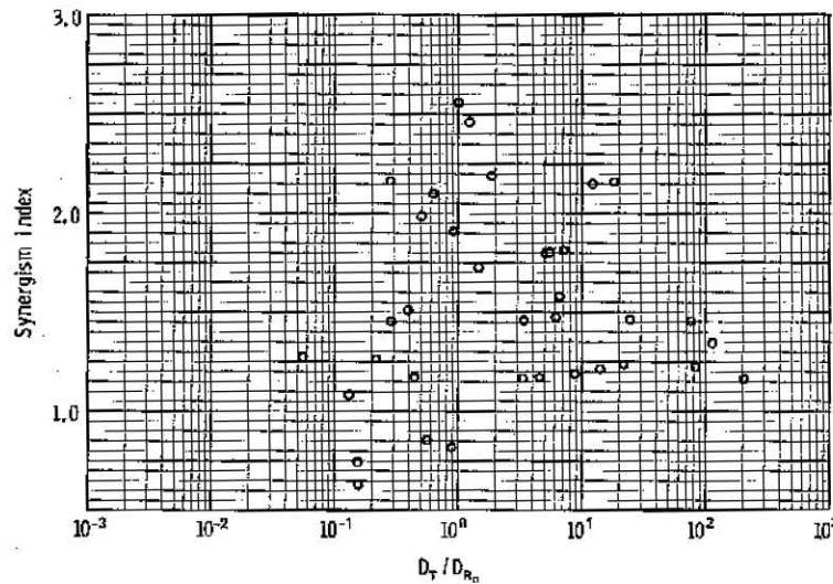
FIG. 5. Values of SI calculated from experimental dry-heat thermoradiation study.
