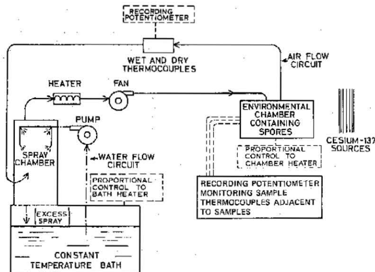
FIG. 2. Schematic flow chart for the environmental system in thermoradiation experiments.
